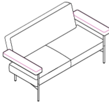
TI2BN L: 1640 P: 830 HT: 810 HS: 420 HB: 610
