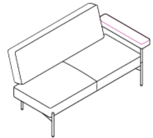
TI2SN L: 1560 P: 830 HT: 810 HS: 420 HB: 610
